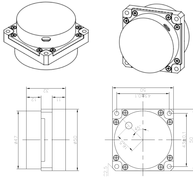
Figure 1 FG-50 fiber-optic gyroscope outline and installation schematic
