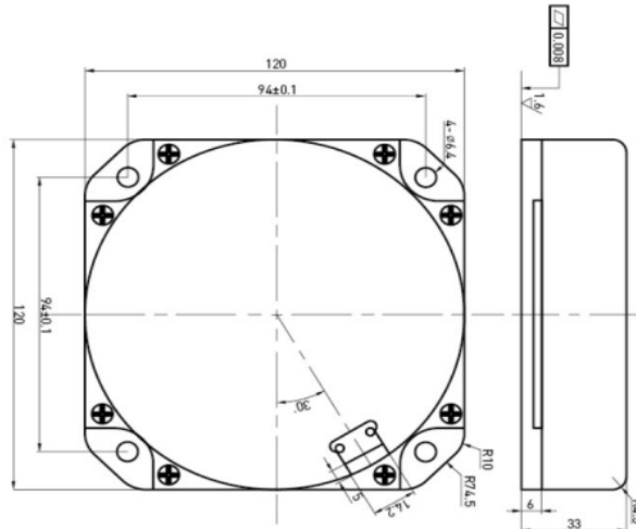
Figure 1 FG-120 fiber-optic gyroscope outline and installation schematic
